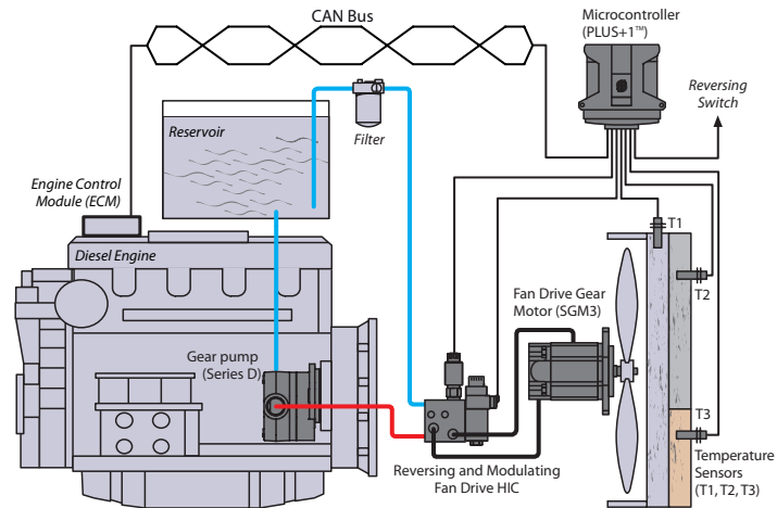
Gear pump/gear motor with electro-proportional relief valve
