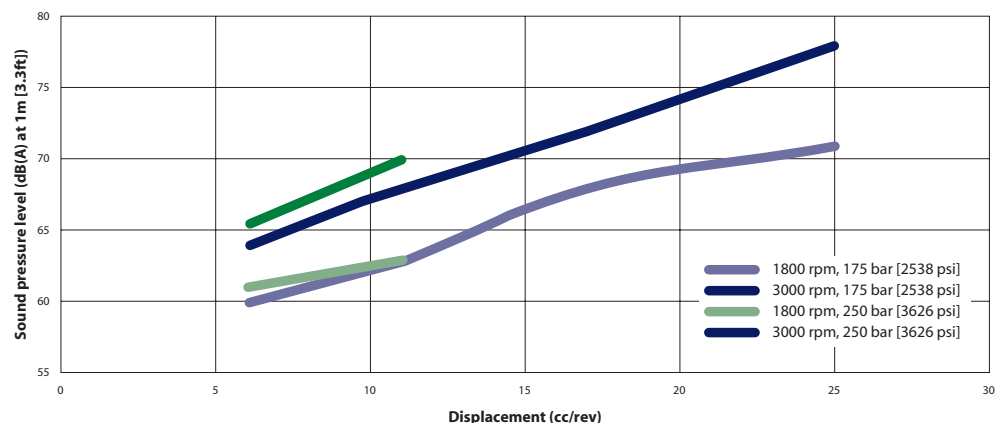
Sound levels graph
