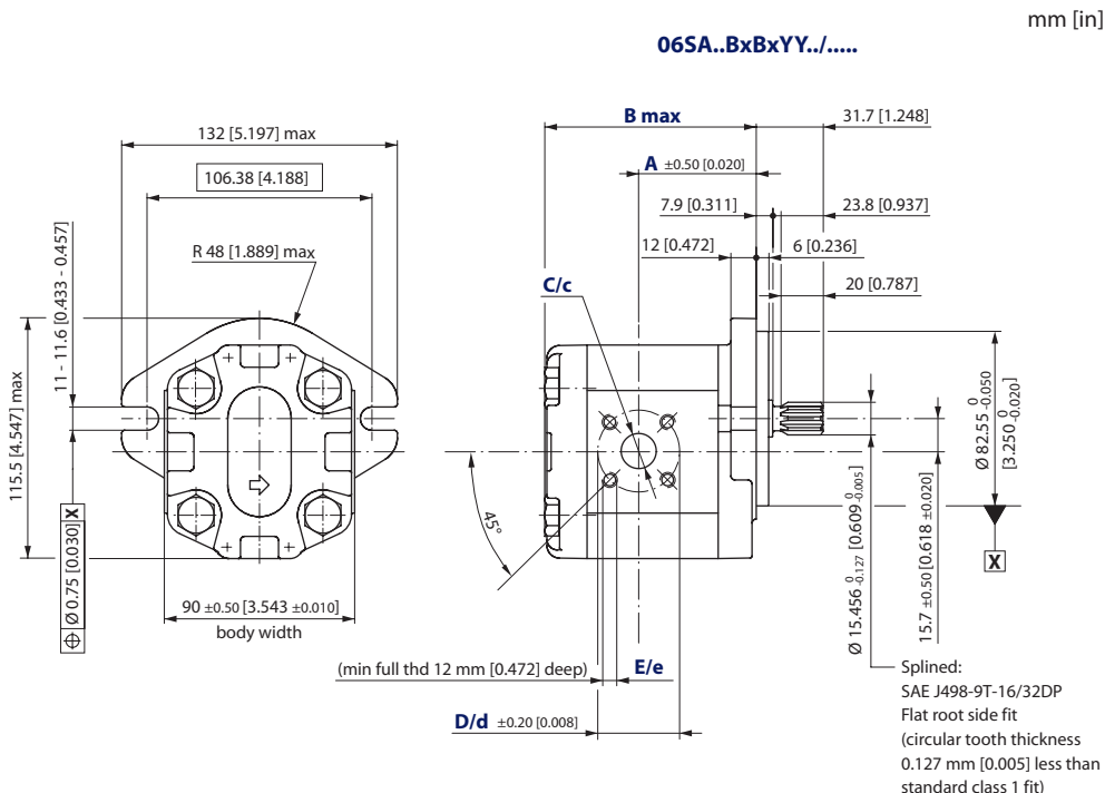
SNP2NN – 06SA..BxBxYY../..... dimensions
