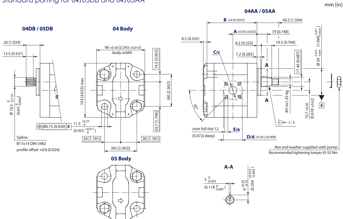
SNP2NN – 04/05DB and 04/05AA dimensions
