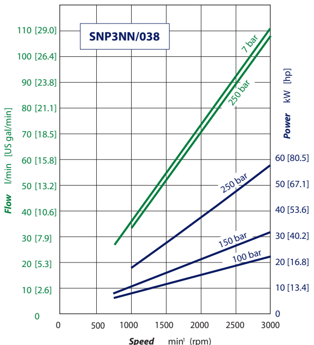
SNP3NN/038 pump performance graph
