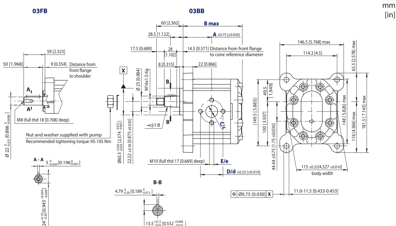
SNP3NN – 03FB and 03BB dimensions
