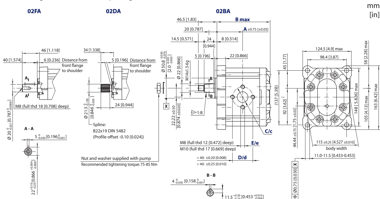
SNP3NN – 02FA, 02DA and 02BA dimensions
