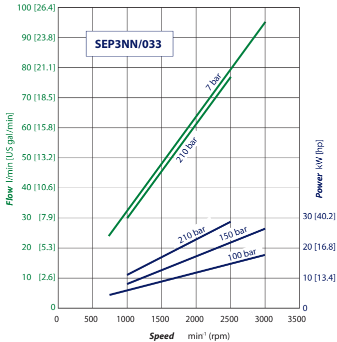
SEP3NN/033 pump performance graph
