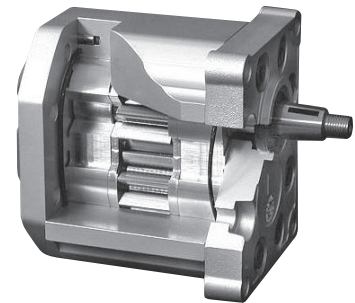
SNP3NN 01BA (cut away)
