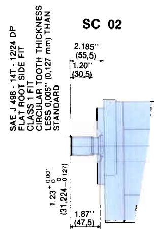
Splined shaft
