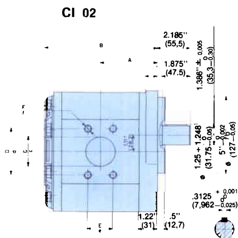
Parallel Shaft
